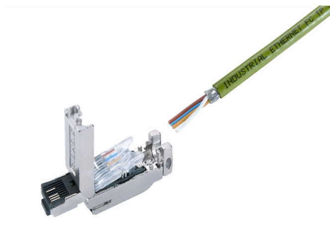
Figure 4-6 IE FC RJ-45 Plug 180
