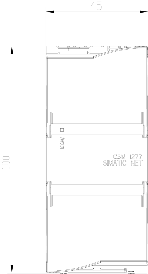
Figure 8-1 Dimension drawing, view from above
