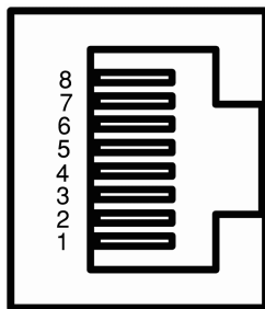
Figure 3-3 RJ-45 jack
