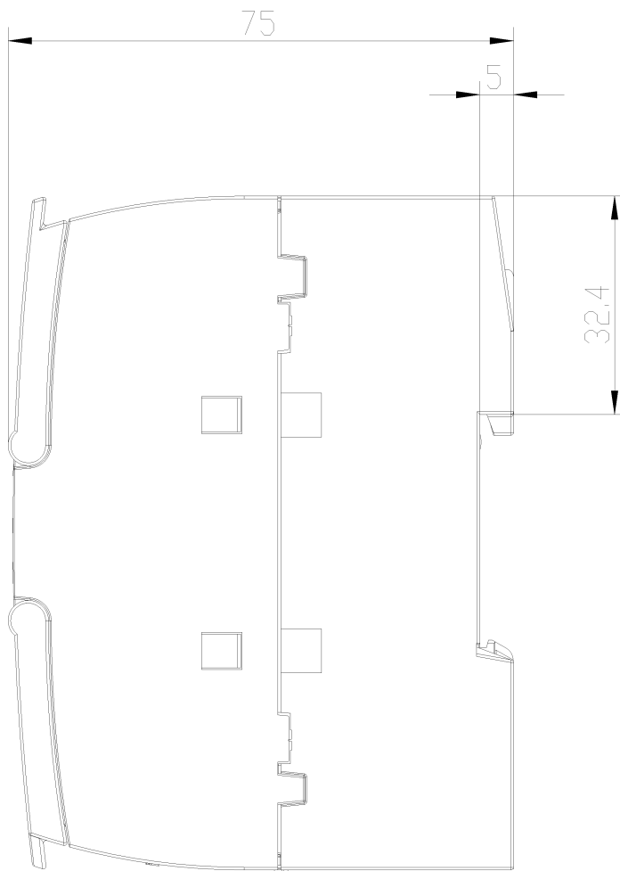
Figure 8-2 Dimension drawing, view from side
