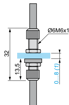
End fitting for passing through partition
