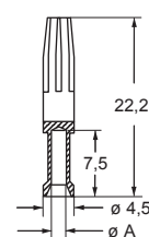
RCF2D and RCM2D contacts
