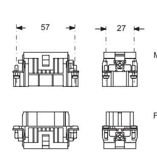
contacts side (front view)
