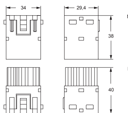
contacts side (front view) side with reference arrow ▲
