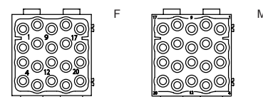
- 2 frame slots
