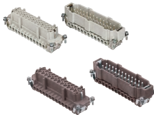
CNE...RY variant
