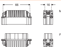
contacts side (front view)
