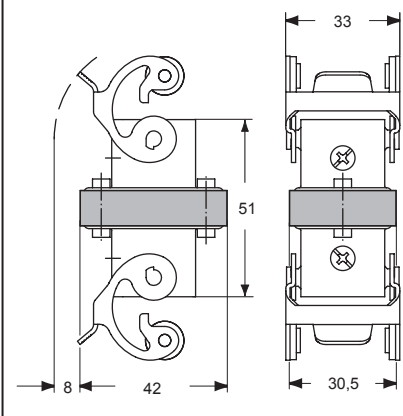
CYG 4 JFA, CYG 4/2 JFA, CYG 8 JFA, CYG 8/2 JFA
