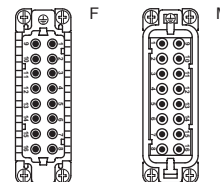
contacts side (front view)
