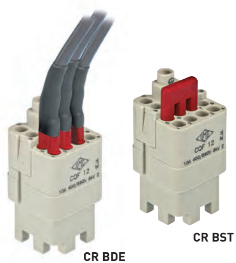
CR BDE
