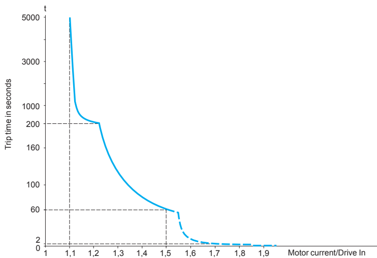
Drive thermal protection curves
