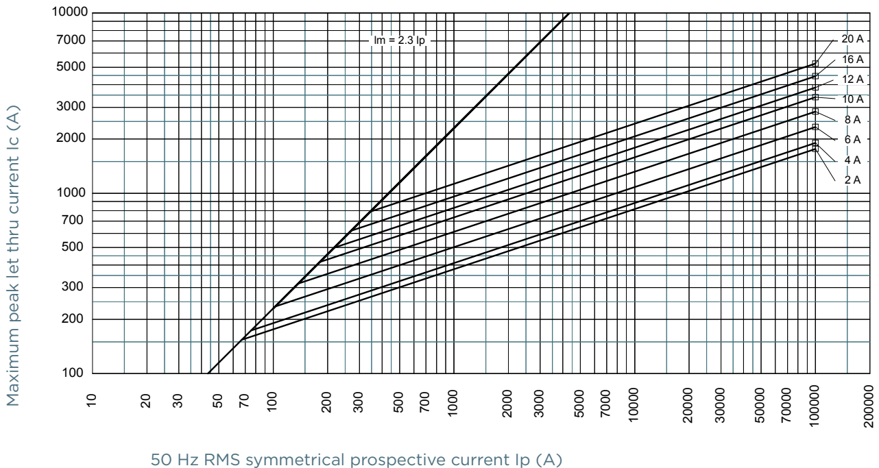
Size 10x38 400V aM with striker 50 Hz RMS symmetrical prospective current I p (A)
